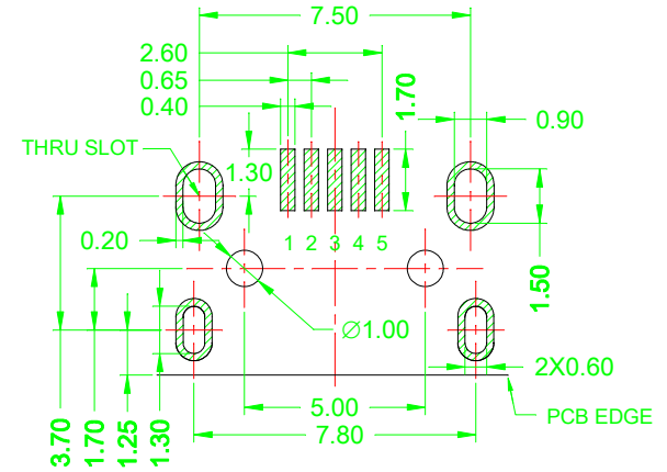
RECOMMENDED PCB LAYOUT (PCB T=1.60mm)
