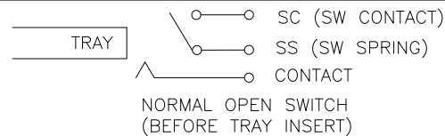
MSD CARD ELECTRICAL
