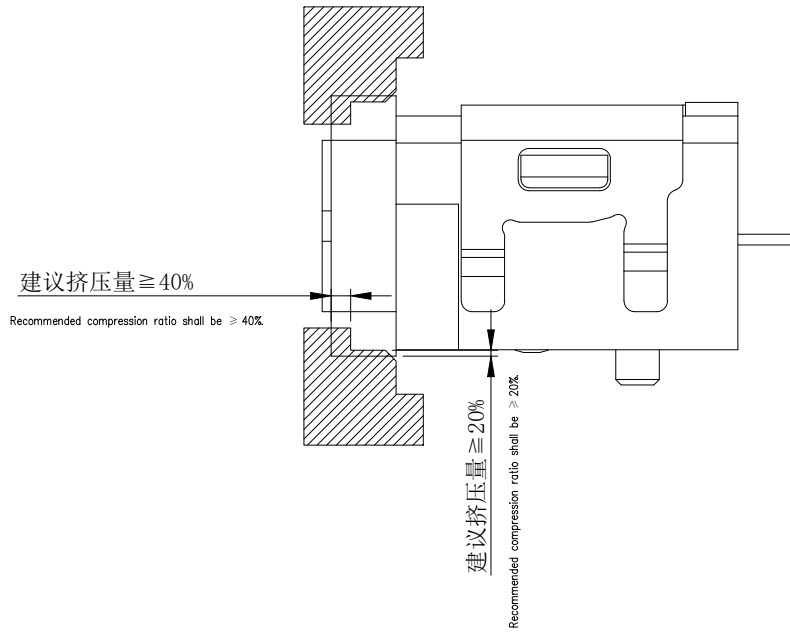
RECOMMENDED SCHEMATIC DRAWING OF CONNECTOR MATCH CHASSIS
