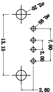
PCB LAYOUT
