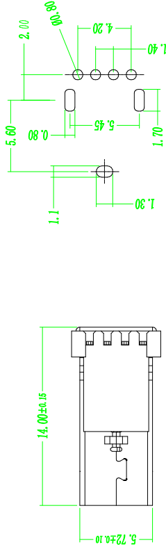
PCB LAY-OUT (BOTTOM VIEW)
