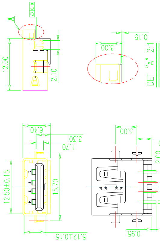
RECOMMENDED P.C.B. PATTERN LAYOUT
