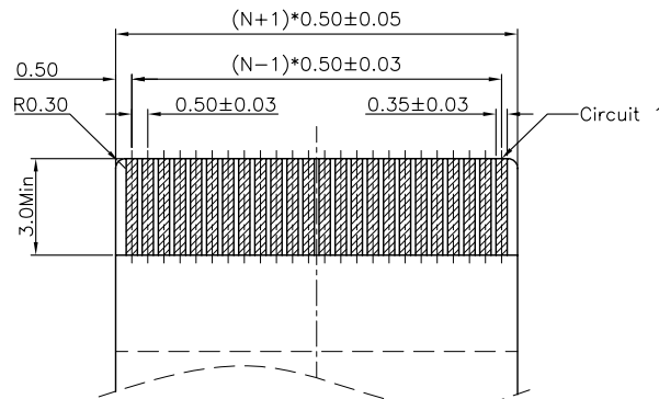
RECOMMENDED FPC/FPC DIMENSION
