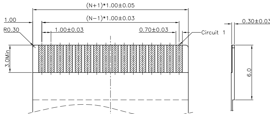
RECOMMENDED FPC/FPC DIMENSION
