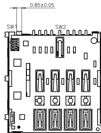
DETECT SWITCH
